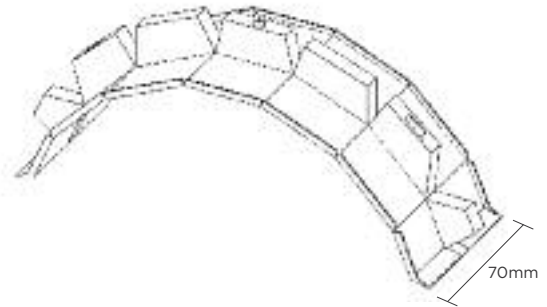
Clamping plates
