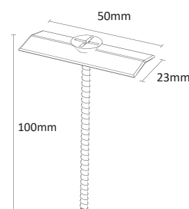
Screw and clamping plate
