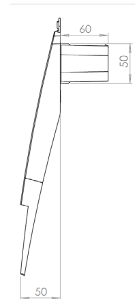
Side Profile
