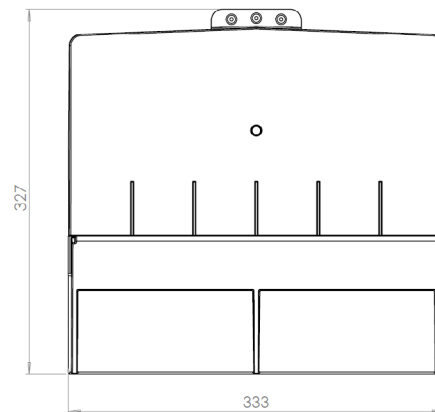
Top Profile
