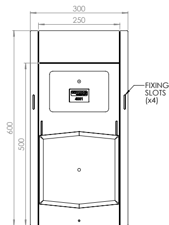
Top Profile
