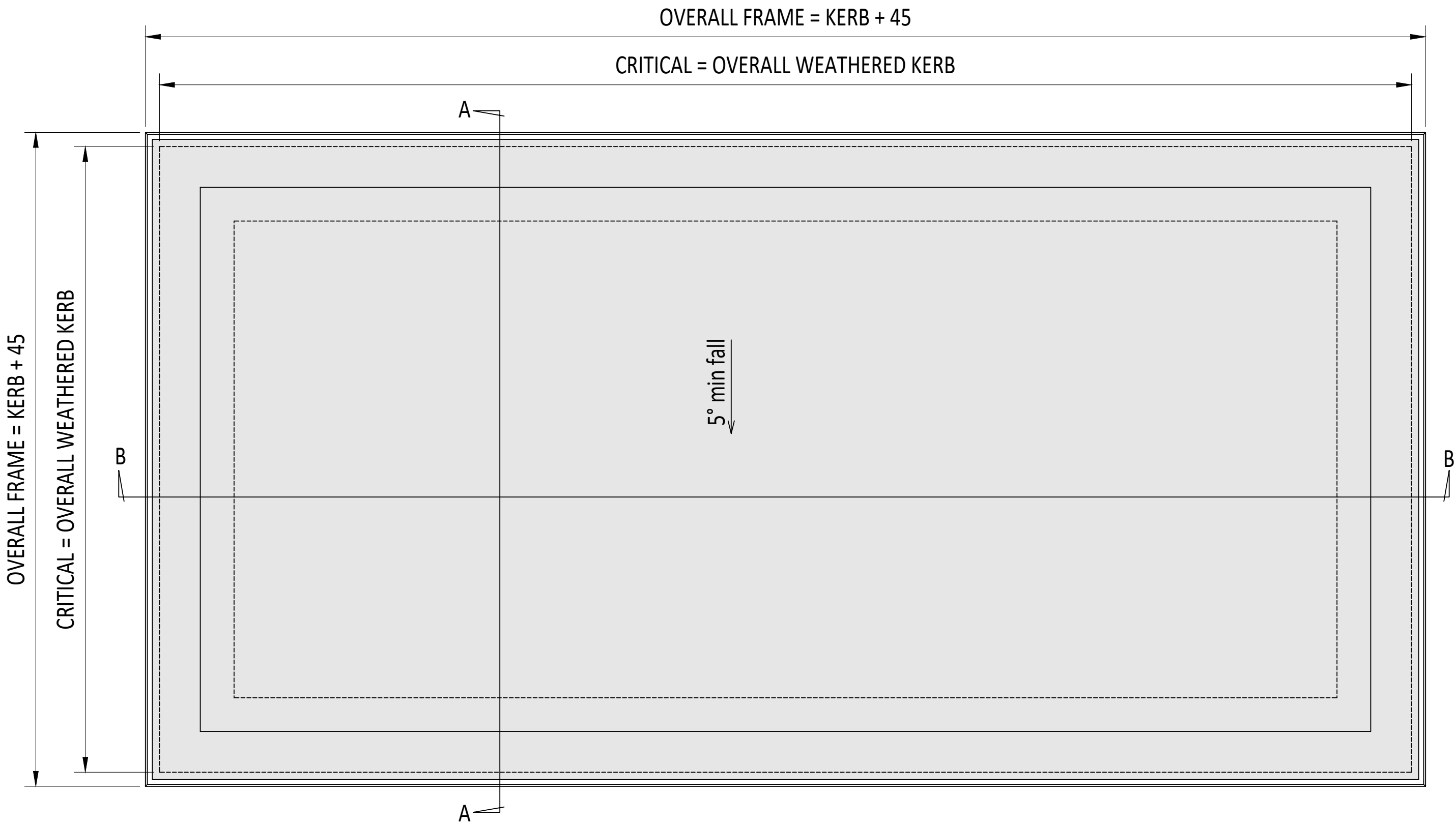
EXTERNAL PLAN VIEW TRUE VIEW ON SLOPE
