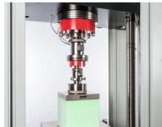
Compression test
