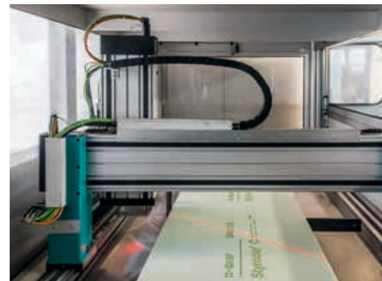
Measurement robot
