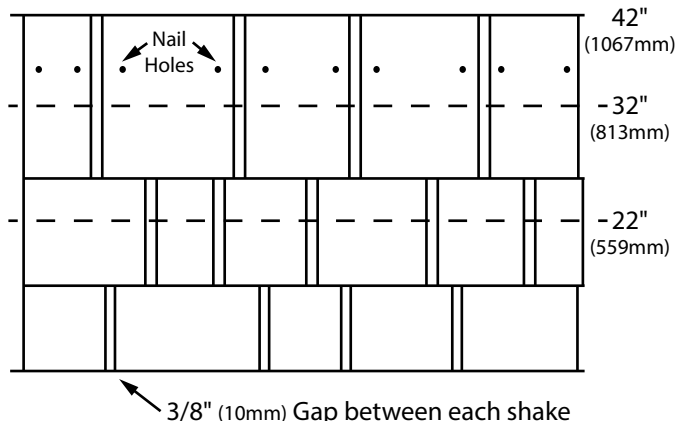
Straight Coursing on Select Shake at a 10" (254mm) Exposure
