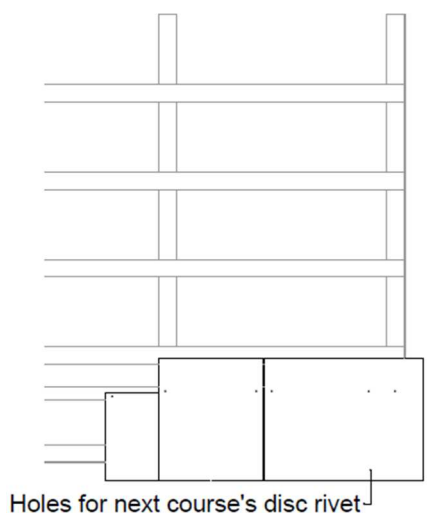
Fig. C - Eaves: 2nd under eaves course
