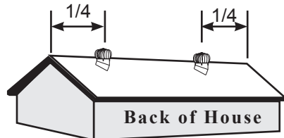
Proper Spacing With Two Whirlybird® Turbine Vents Installed
