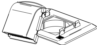
Full Hood Cowl Vent inc. Large backplate with 5" (127mm) Spigot Brown, Terracotta, White
