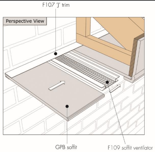
vented soffit joiner detail — perpendicular
