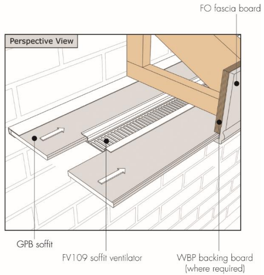
vented soffit detail — parallel
