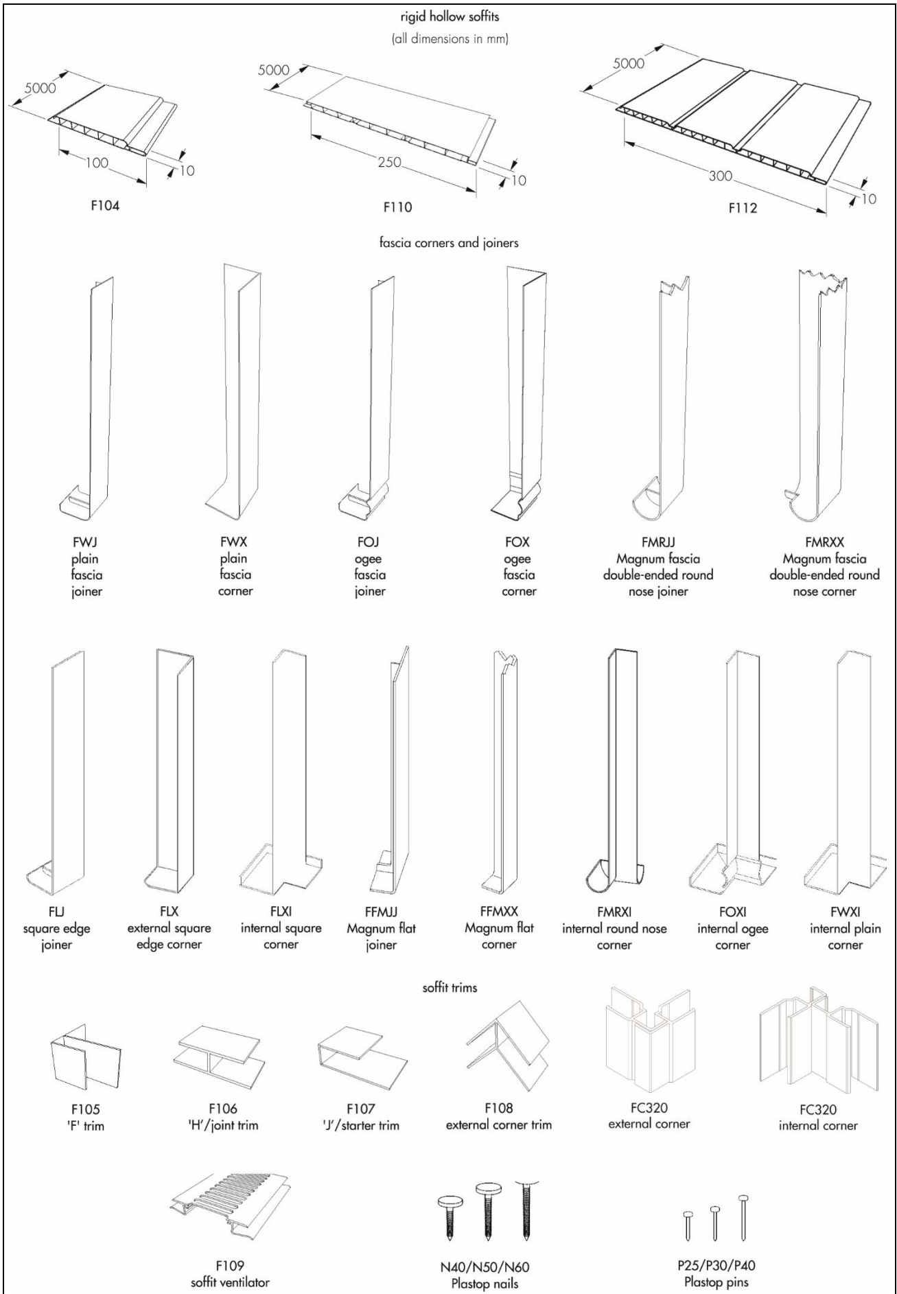
Figure 2 Ancillary components
