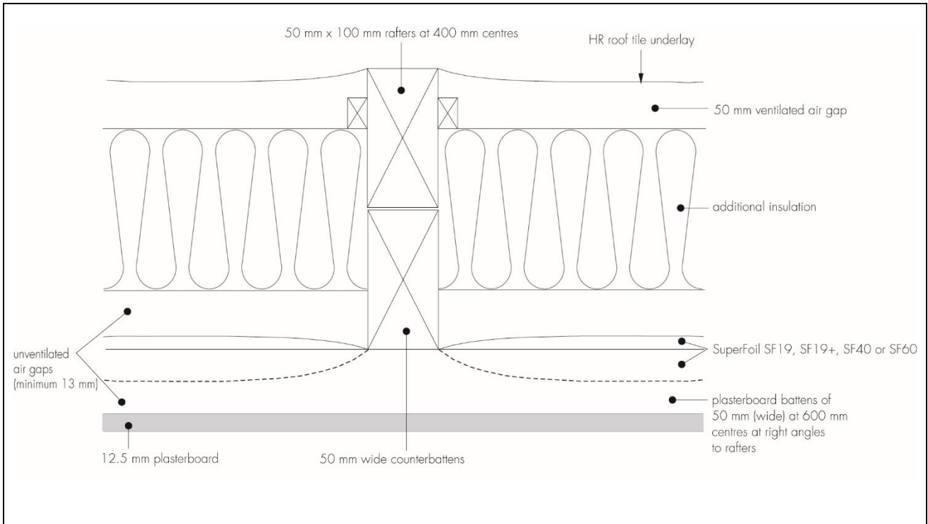
Figure 1 Example pitched roof constructions — existing roof — refurbishment
