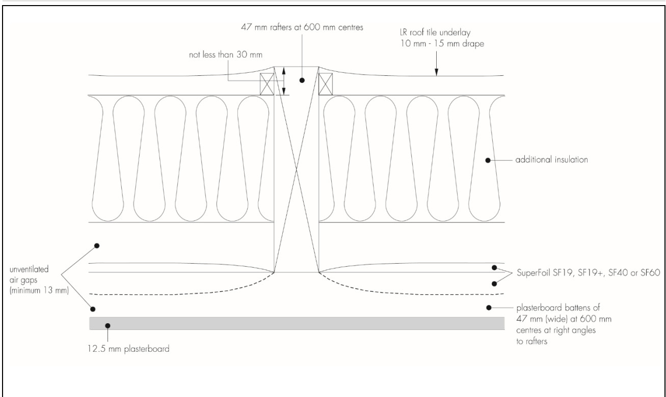
Figure 2 Example pitched roof constructions — new build
