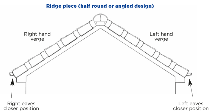
Dry Fix Verge System For Profiled Roof Tiles - Grey
