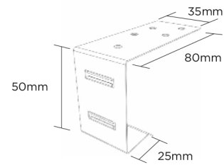
Dry fix verge angled ridge/apex piece
